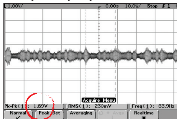
Shaft voltage with carbon fiber grounding ring
