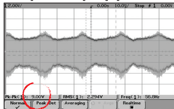
Shaft voltage with carbon fiber grounding ring
