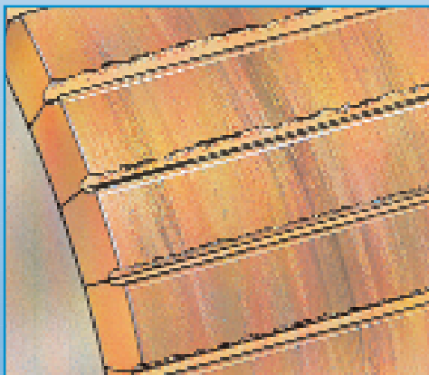
Damaged Commutator
